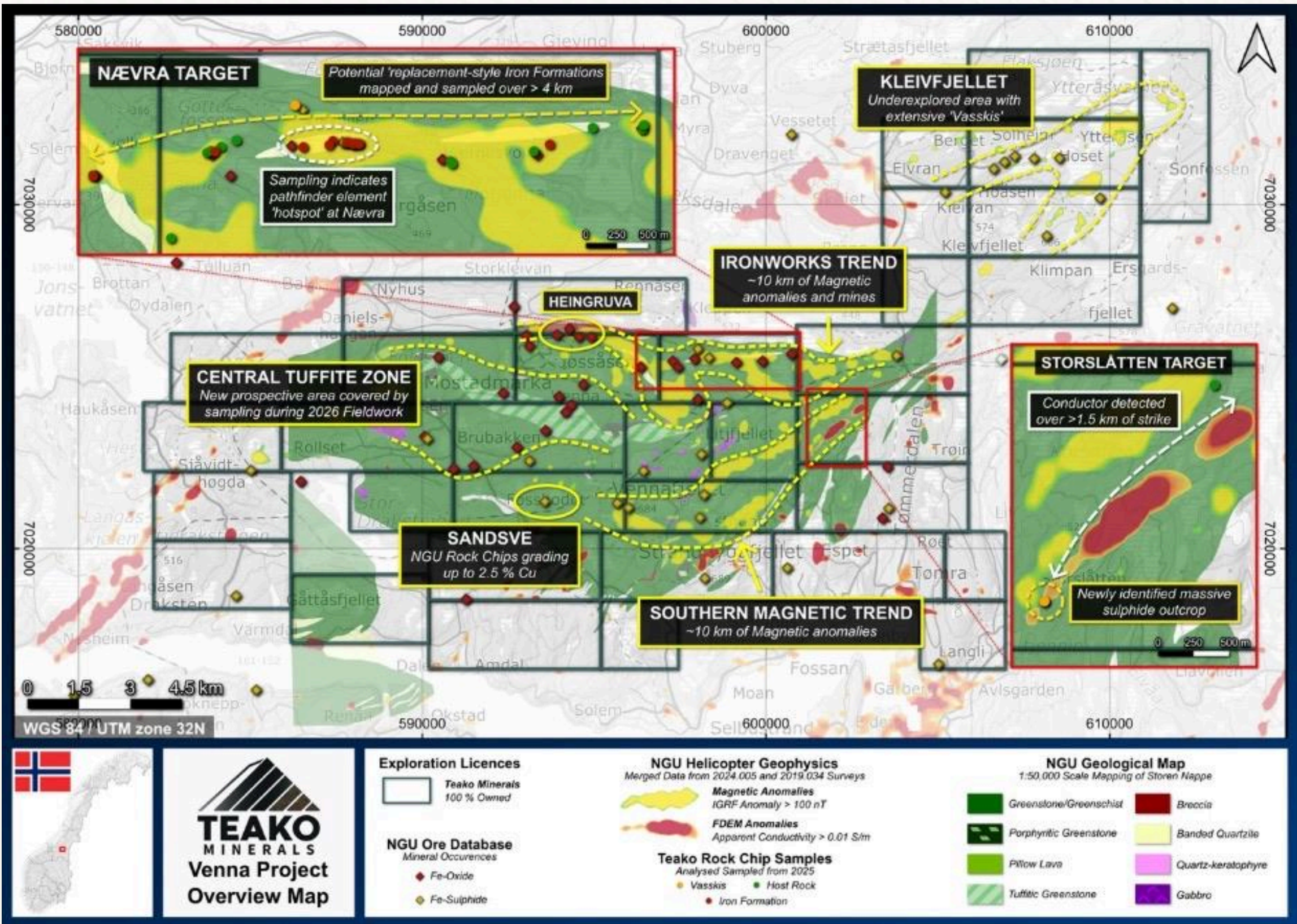
FIG. 17 · VENNA TARGETS OVERVIEW
