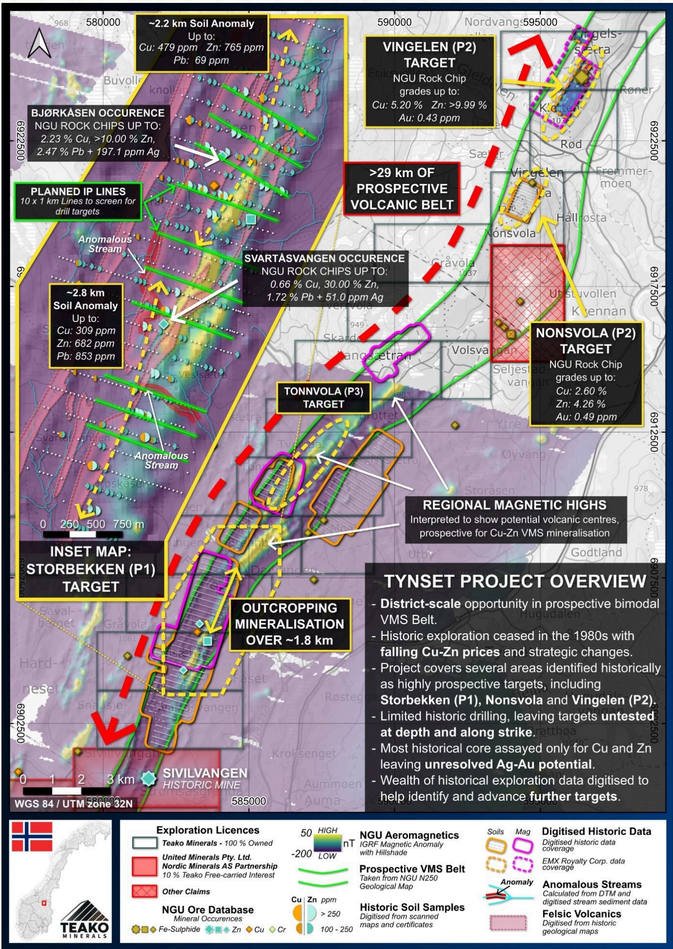
FIG. 13 · TYNSET TARGETS OVERVIEW
