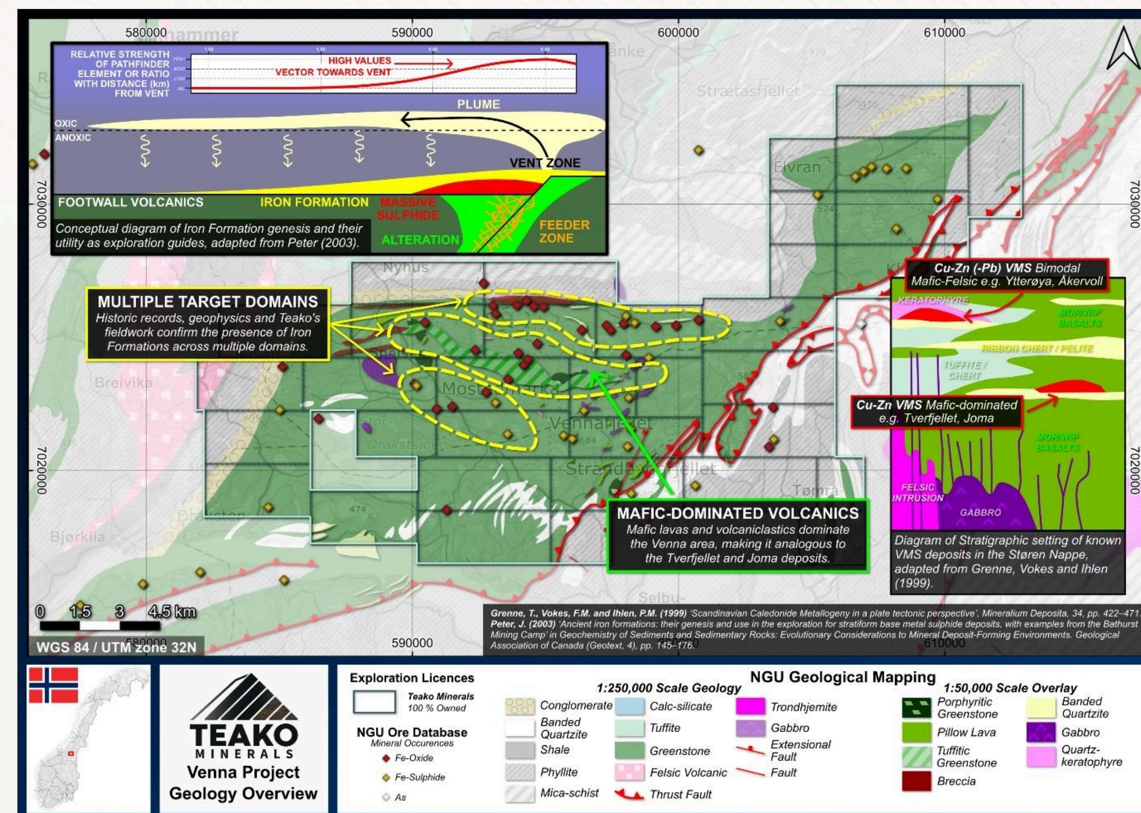
FIG. 16 · VENNA GEOLOGY OVERVIEW
