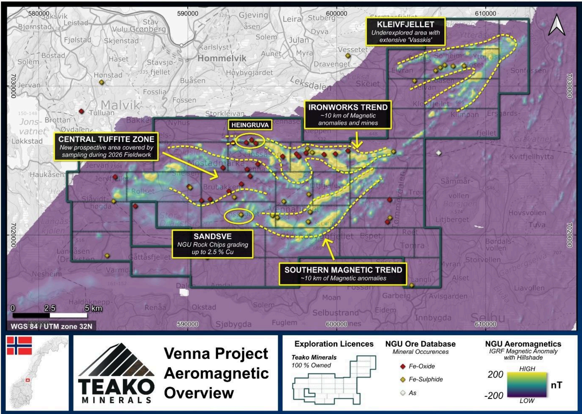
FIG. 15 · VENNA AEROMAGNETIC OVERVIEW
