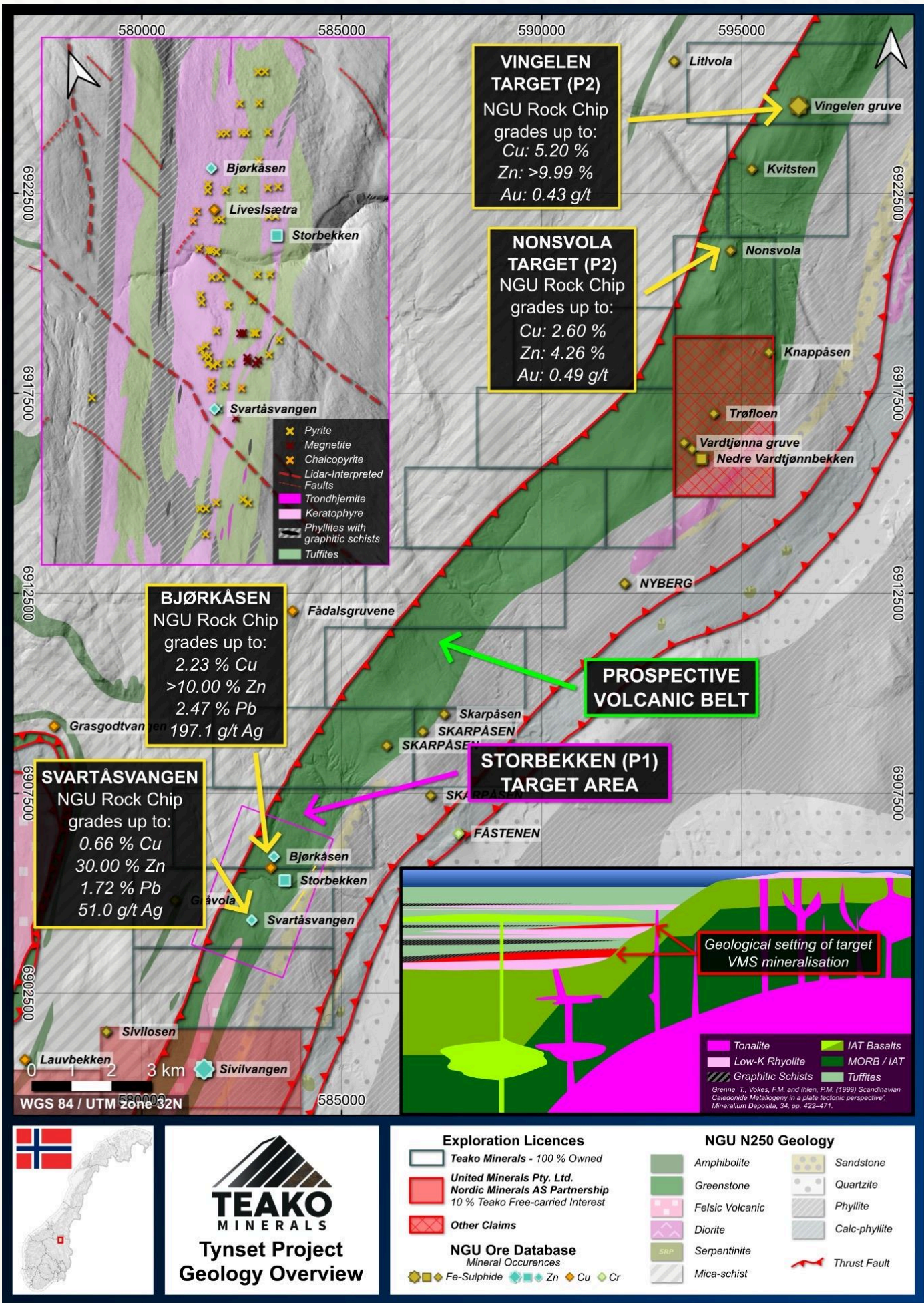
FIG. 11 • TYNSET GEOLOGY OVERVIEW
